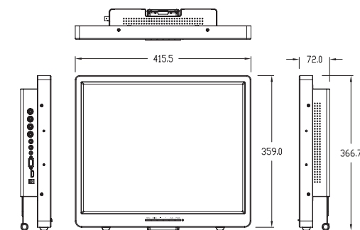
A19M1-LED Dimension
